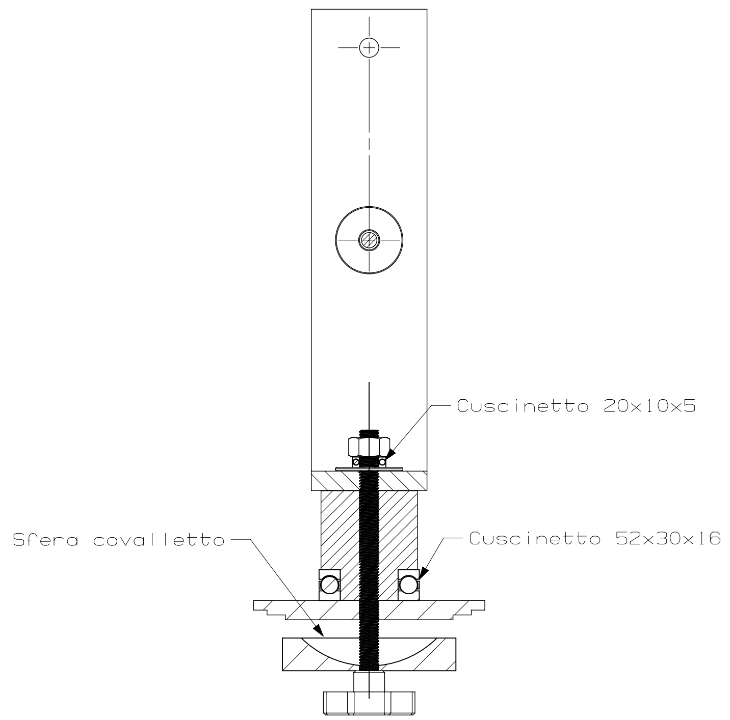
SECTION G-G
